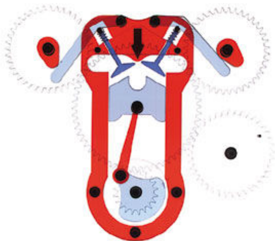
Diesel engine
